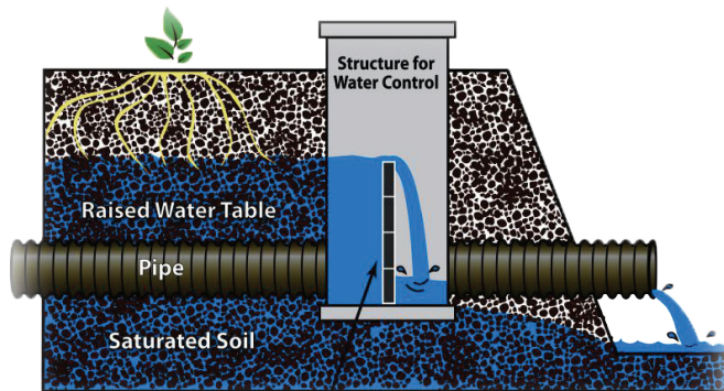
Flow Control Mechanism Illustration Courtesy of NRCS
